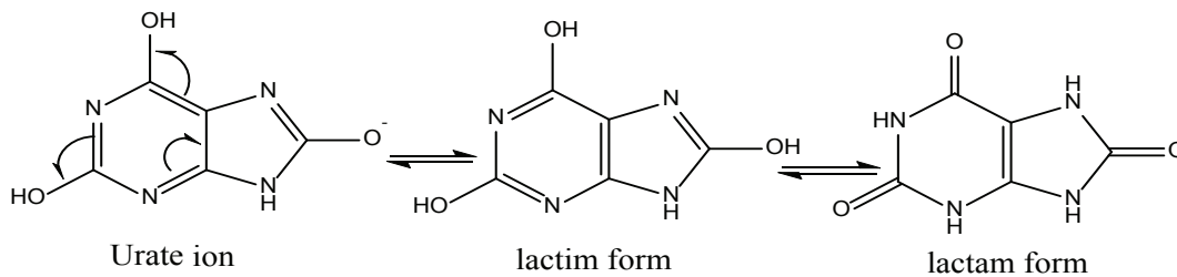
Fig. 3: Urate tautomerism
